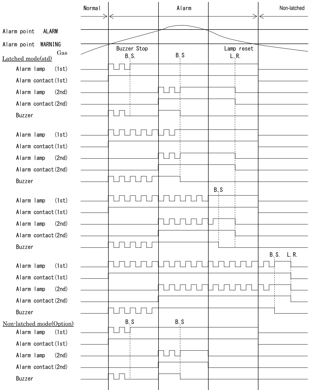
Timing chart
